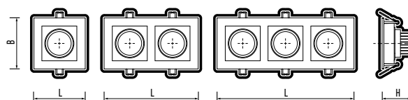
PSP-S 211 1x8W
