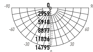
PWW 1000 24W
