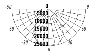
PFL-S4 300W
