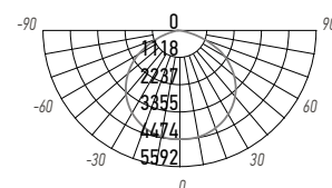
PFL-C3 150W
