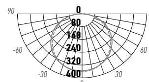
PBH-PC7-RS 12W
