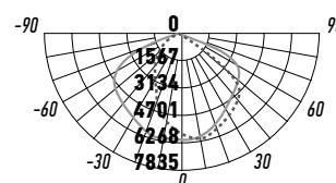
PSL 09 150W
