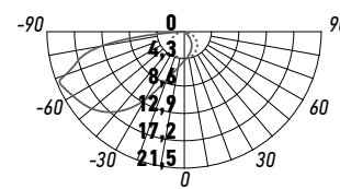
PST/W S120090 2W
