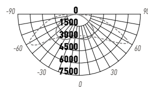
PSL 02 100W
