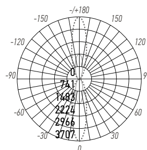
PWL-300110/30D 2X9W
