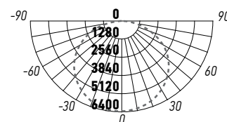
PHB 03 PRO-5 100W
