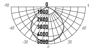
PGL 05 60W
