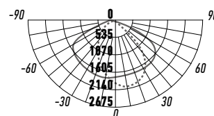
PSL 09 50W
