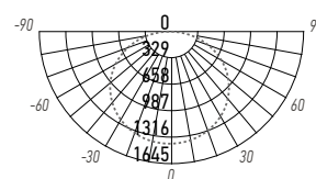
PP0-02 1200 PRISMA 36W
