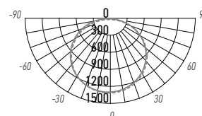
PP0-06 50W
