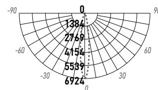
PWW 500 12W
