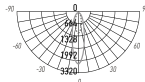
PWL-200110/30D 1X9W
